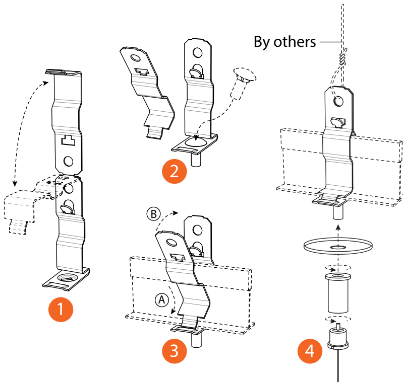
T-Bar ceiling cable coupler kit
