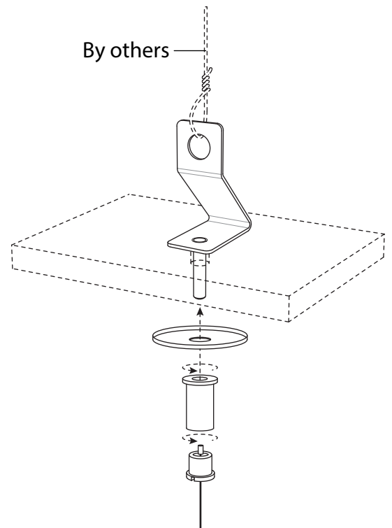
Suspended ceiling cable coupler kit
