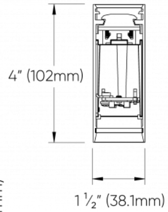
FIXTURE CROSS SECTION
