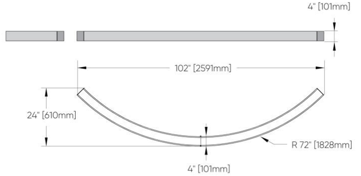
72" Radius
