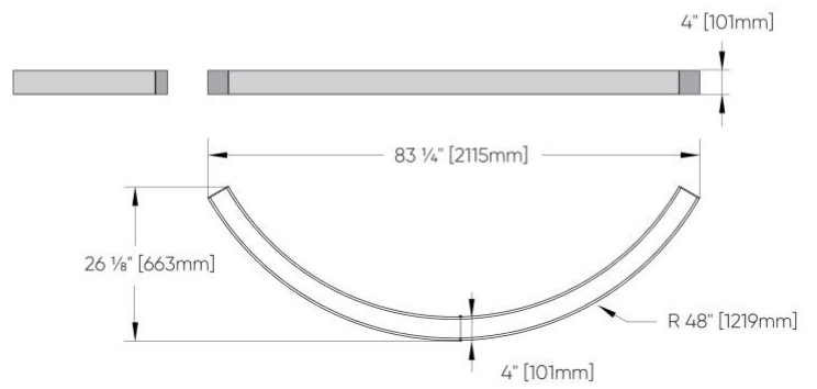
48" Radius
