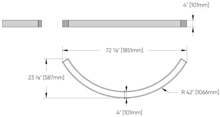
42" Radius
