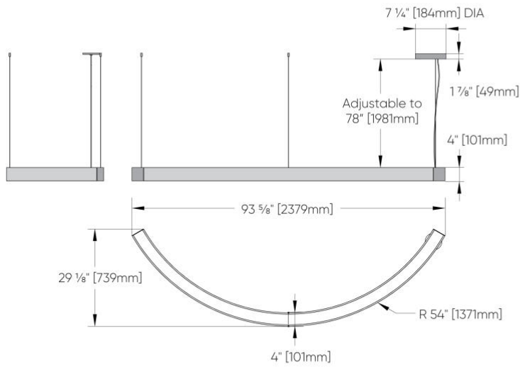
54" Radius
