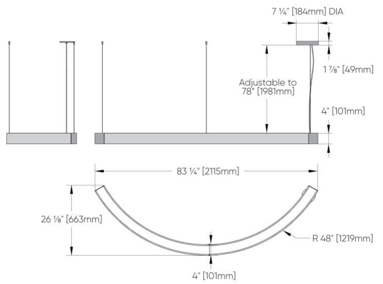
48" Radius
