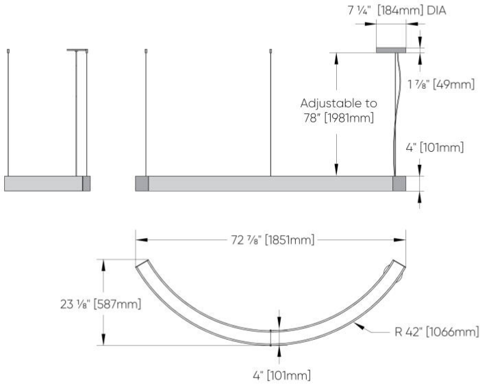
42" Radius
