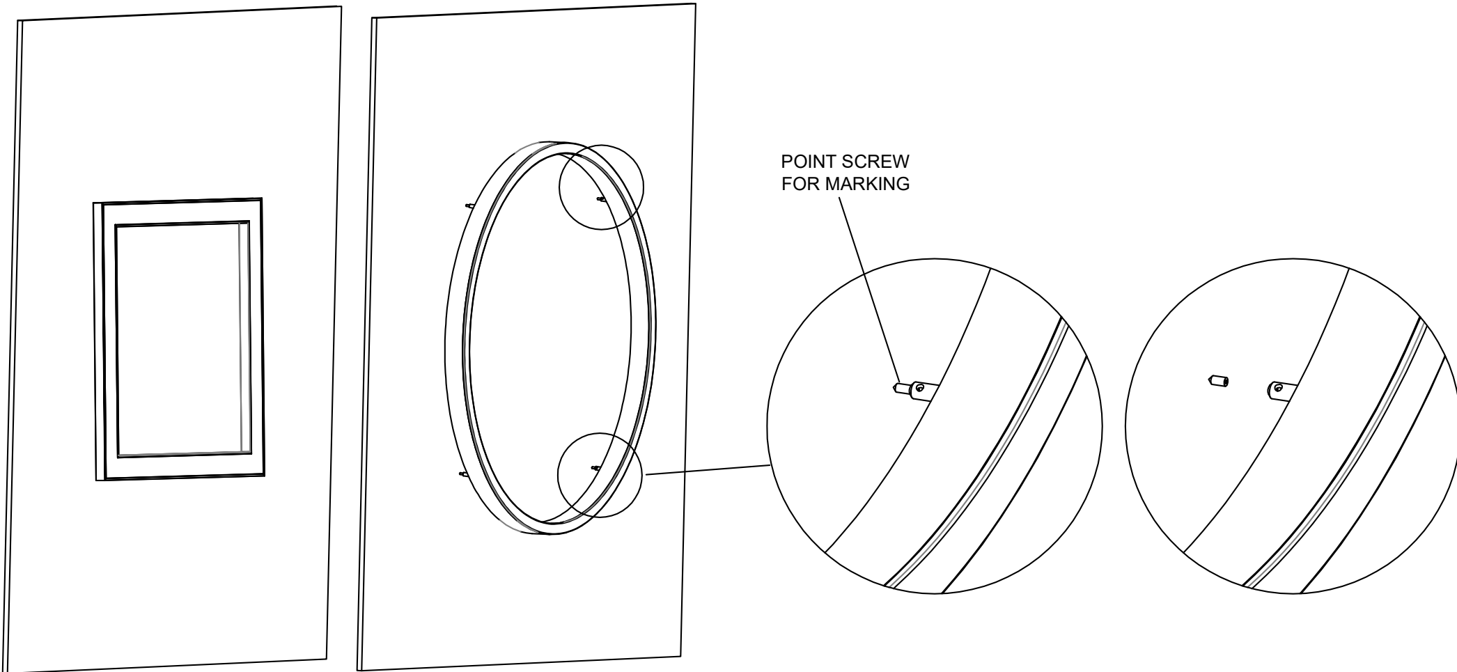
STEP 2 MARK THE MOUNTING HOLES POSITIONS
