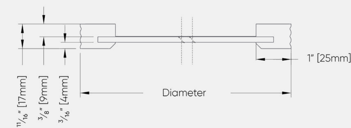
CROSS SECTION
