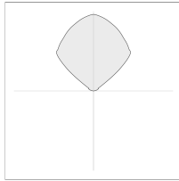
40W-INDIRECT ONLY
