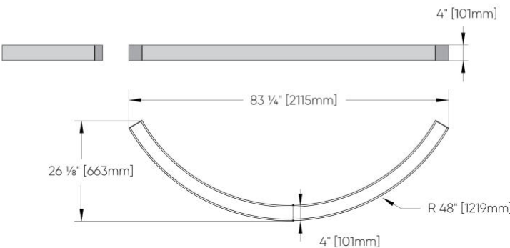
48" Radius
