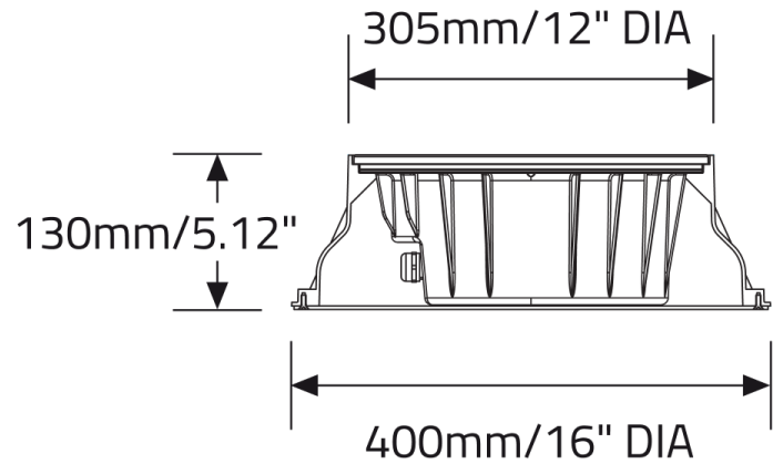
Type B Stainless Steel Bezel
